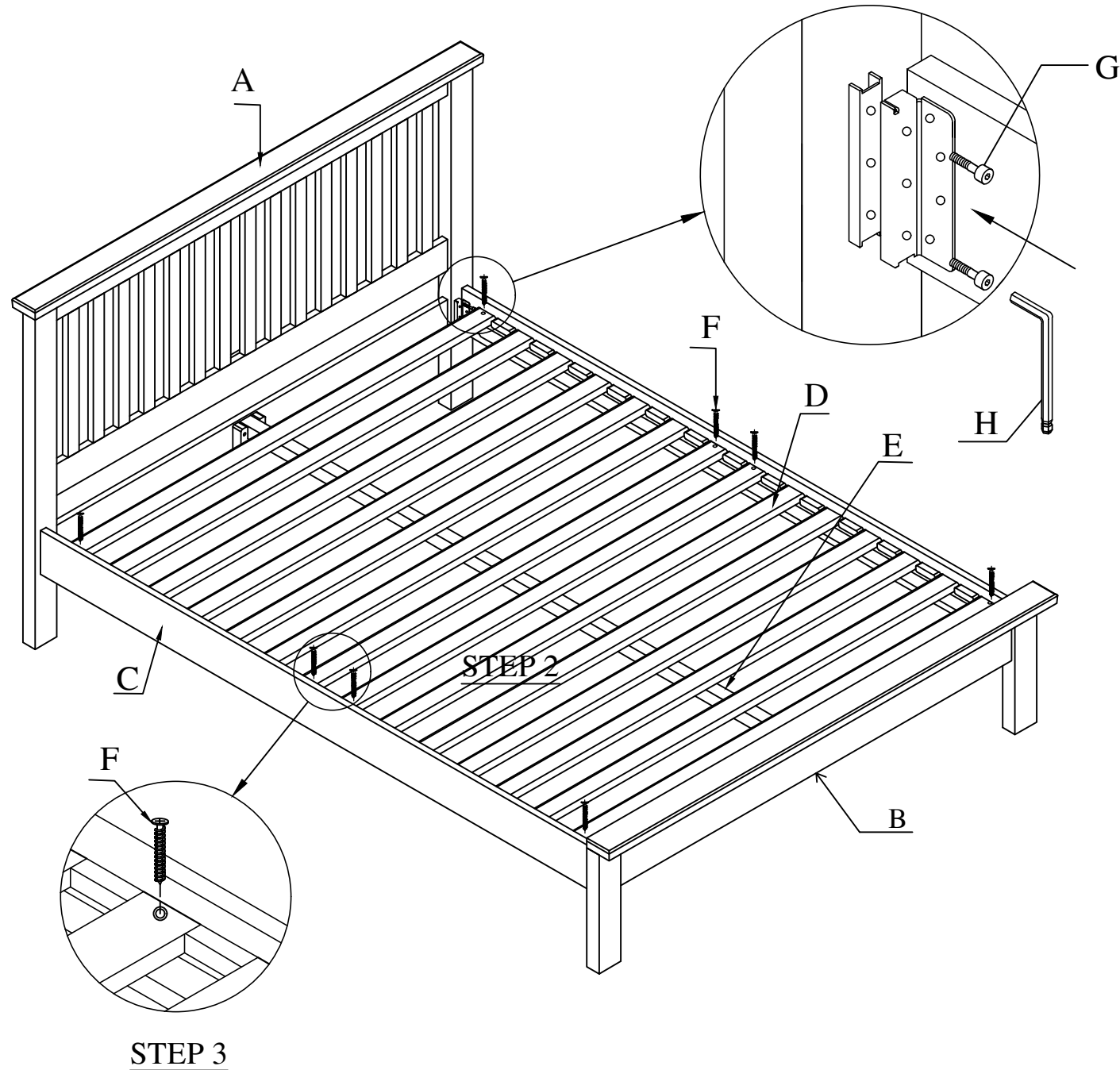
A: Head Board x 01
