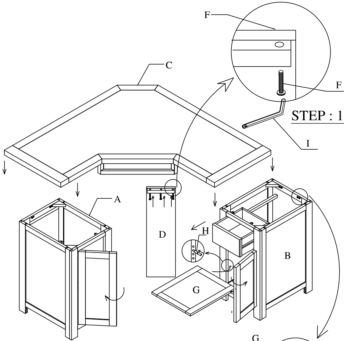
D: BACK FRAME x 01
